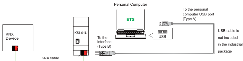
Figure 2: Connection Scheme
